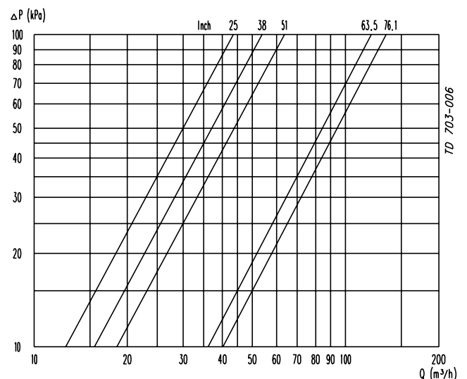
Fig. 2. LKVF with ø2 mm holes in filter element. Medium: Water (20°C).
