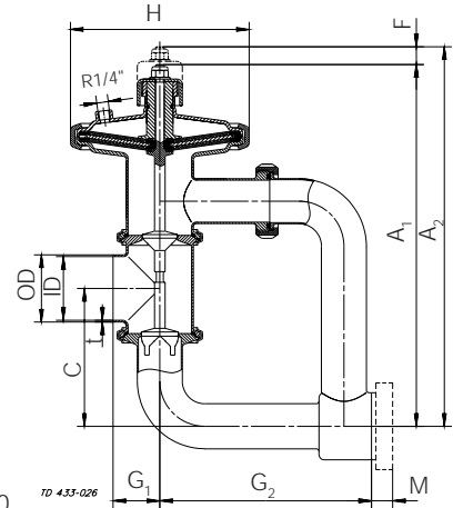
Fig. 4. Dimensions.
