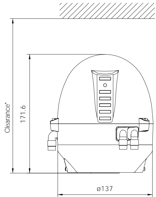
Fig. 3. Dimensions.
